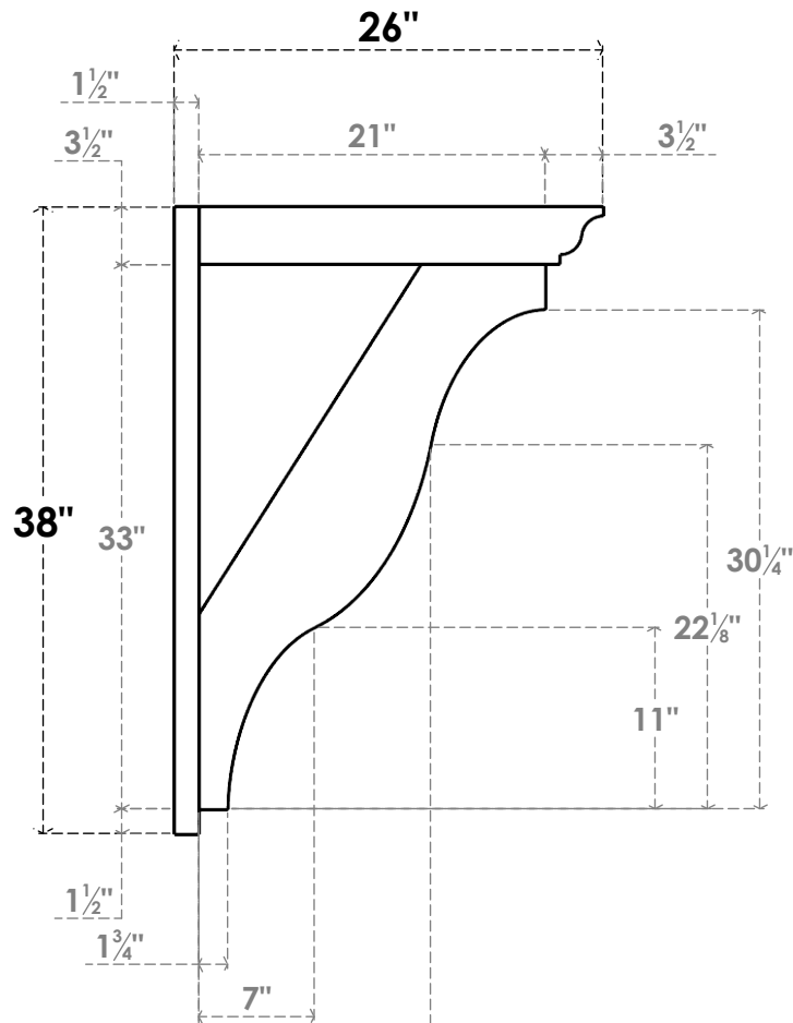
SIDE PROFILE
